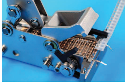
2. Shims and SMD Tape ends inserted in Tool and "rivited" together
